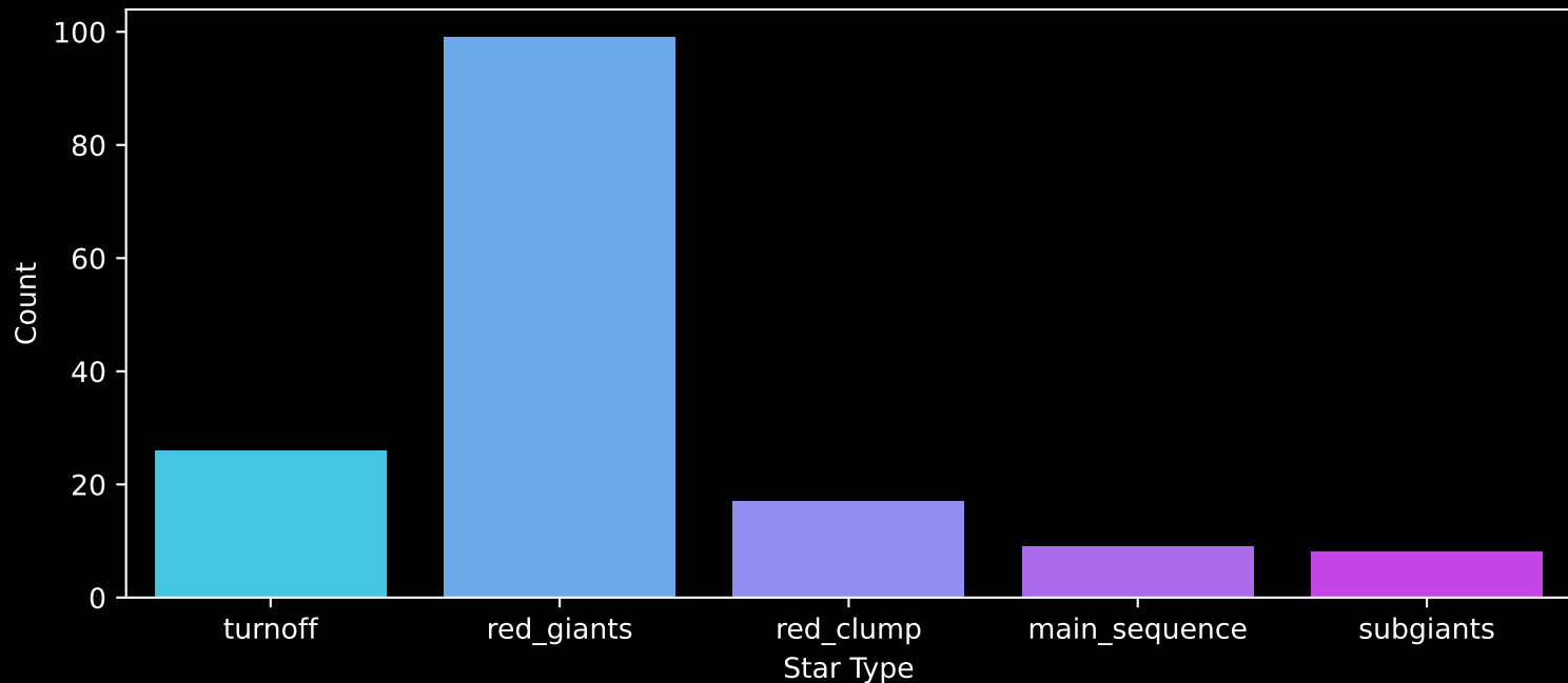
APOGEE DR17 Field: [060+30] Count plot of Star Type
