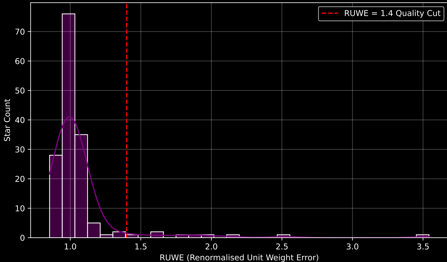
GAPOGEE DR17 Field [060+30] RUWE Distribution (n= 156)
