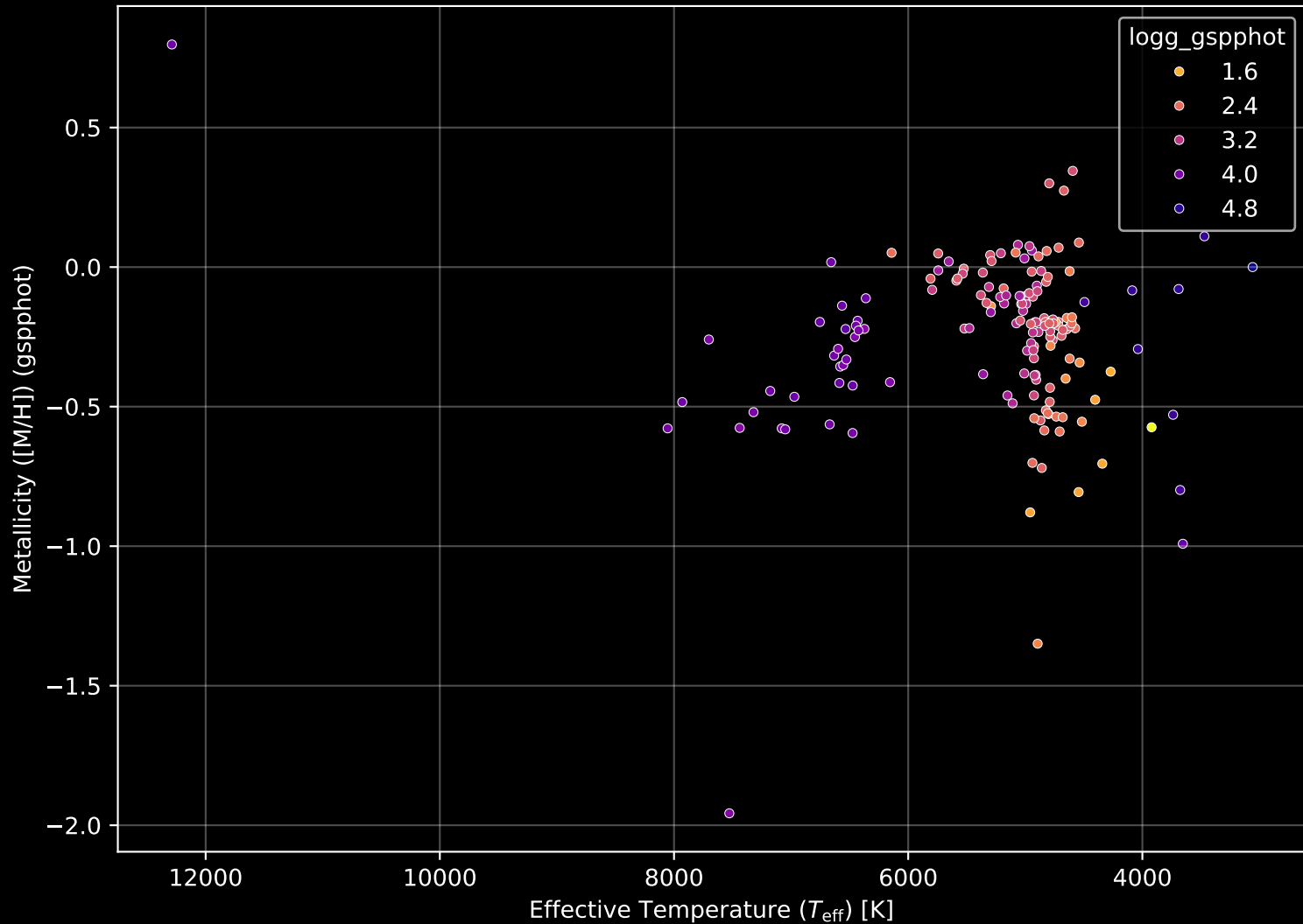
APOGEE DR17 Field: [060+30] Stellar Population Parameters (n= 159)
