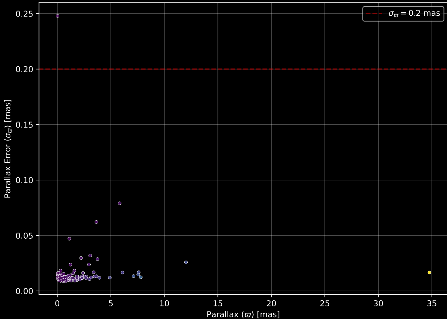
APOGEE DR17 Field: [060+30] Parallax Quality (n= 159)
