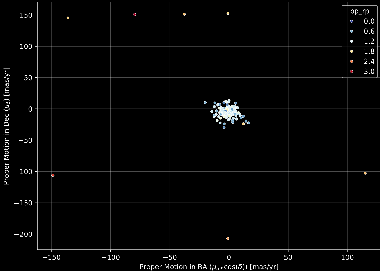
APOGEE DR17 Field: [060+30] Proper Motion Diagram (n= 159)
