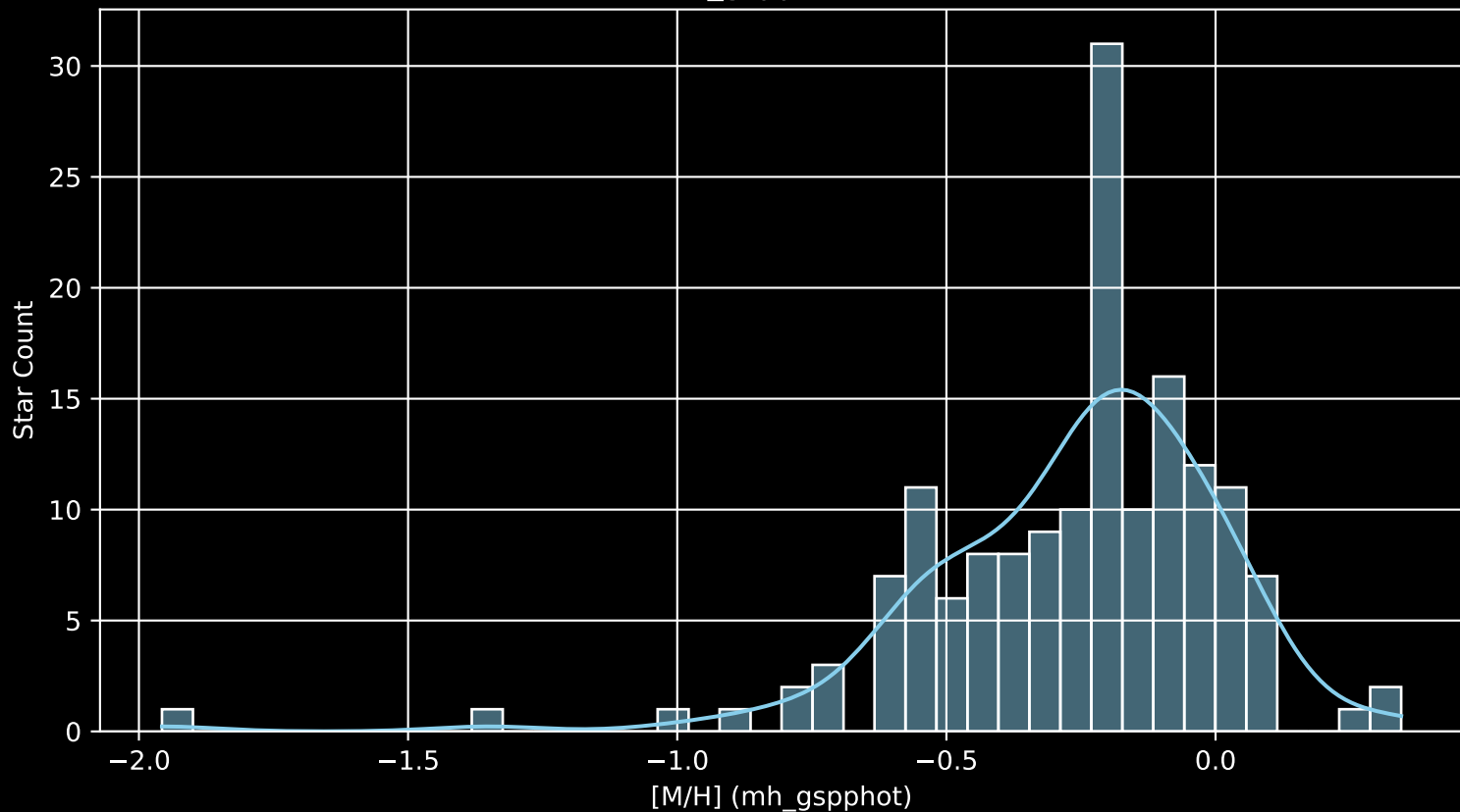
APOGEE DR17 Field: [060+30 [M/H] (mh_gspphot) (n= 158)
